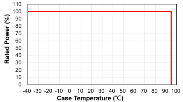
Case Temperature Derating Curve
