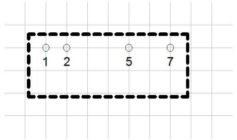
Print board vertical view Grid: 2.54mm(0.1inch)
