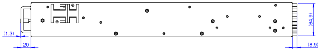
Figure 8. Bottom view
